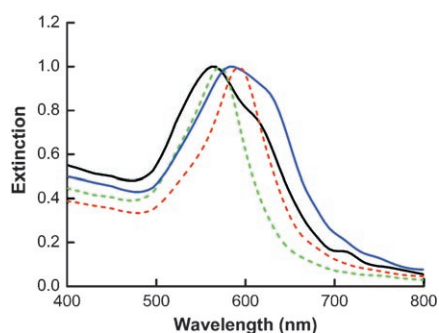
Figure 5. Calculated extinction spectra of Au nanoparticles in ethanol. The black and blue solid traces correspond to nano-octahedra with edge lengths of 30 and 60 nm, respectively. The green and red dashed traces correspond to 30- and 60-nm nano-octahedra, respectively, whose tips are truncated by 3 nm. The peaks are normalized in all traces.
